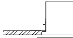
Plasterboard*
